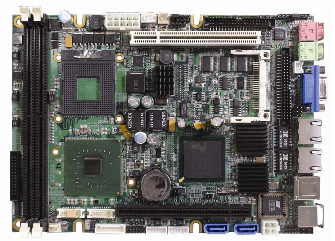
Figure 1.2: Overview of EBC 500
