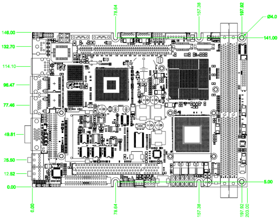
Figure 1.3: Mechanical Drawing of the EBC 500
