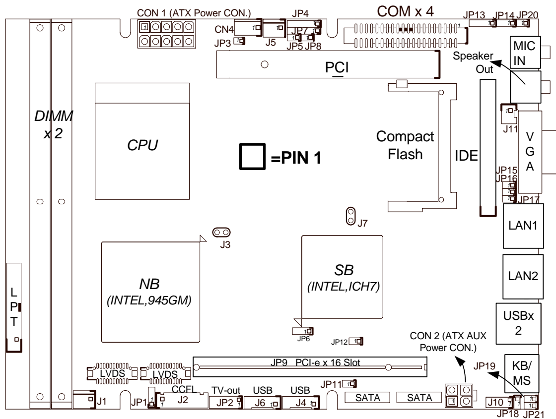
Figure 2-1: Jumper Location
