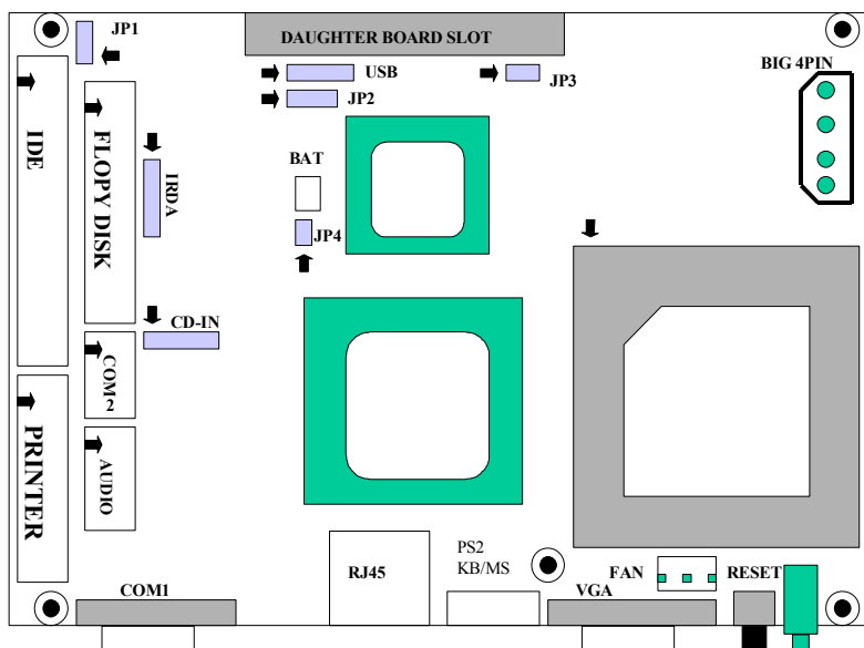
SOLDER SIDE VIEW
