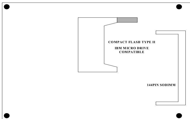
SOLDER SIDE VIEW
