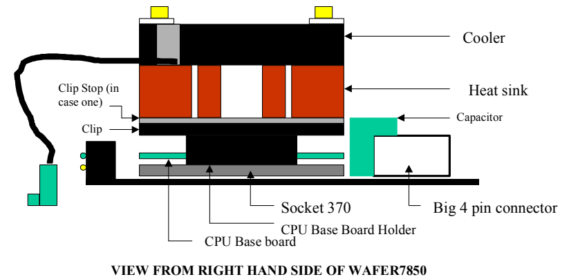
VIEW FROM RIGHT HAND SIDE OF WAFER7850
