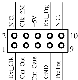
Figure 2.3 Pin Assignment of CN4
